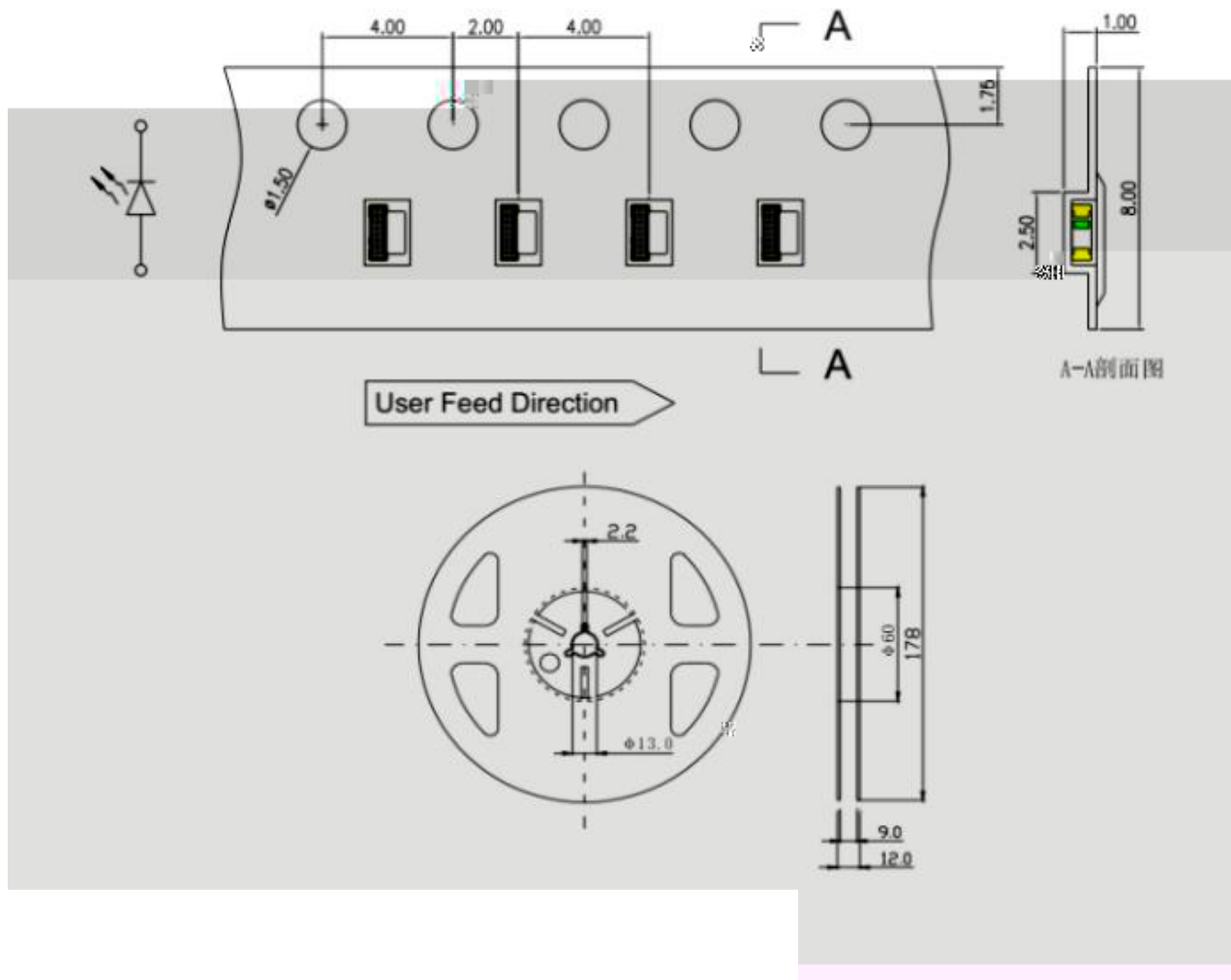
图 1 带盘尺寸 Belt and disk dimensions
